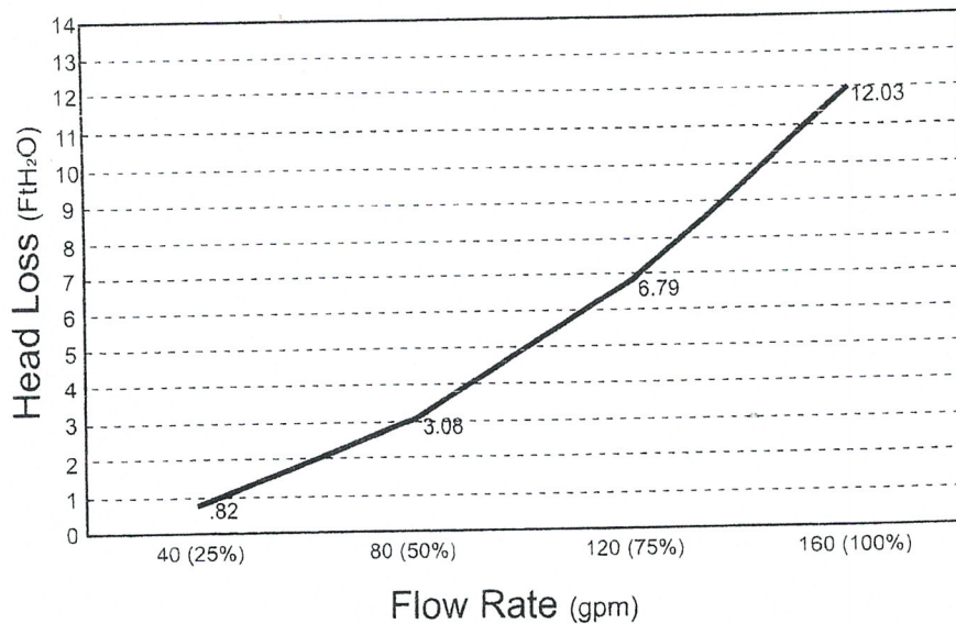
Head Loss Curve
